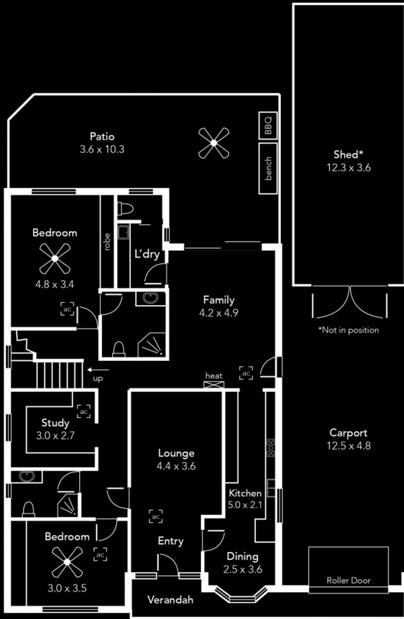
Lower Level
