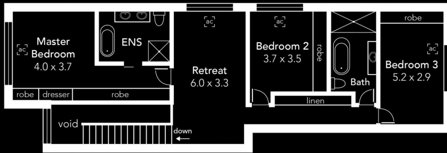
Upper Floor
